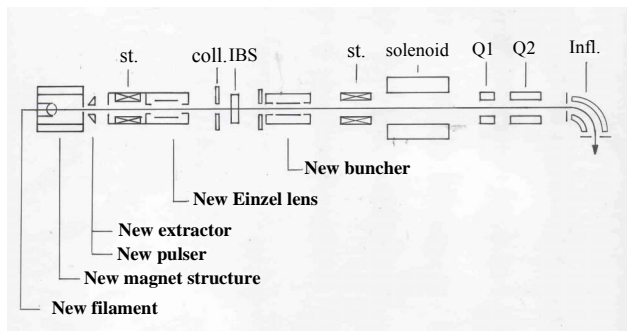
Figure 2: System schematics for source-injection upgrade.
