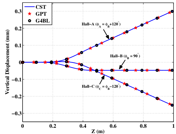
Figure 5: Vertical displacement of an 11 GeV electron for RF phases \phi_A , \phi_B and \phi_C of the superconducting cavity (see Fig. 2). Simulation results are compared using the CST particle tracker, GPT and G4BL (g4beamline) computer codes.
