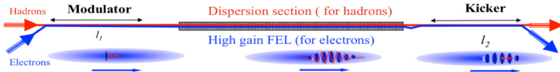
Figure 3: Economic version of coherent electron cooler, wherein electrons and hadrons are not separated transversely.
