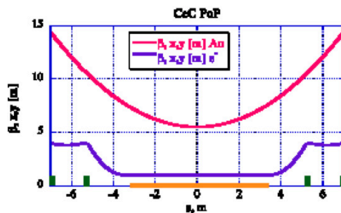
Figure 6: Beta-functions for the ion- (red) and electron-beam (cyan) in the IP2 for our CeC experiment
