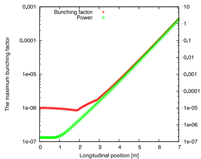
Figure 4: The evolution of optical power (green +) and the bunching factor (red +).
