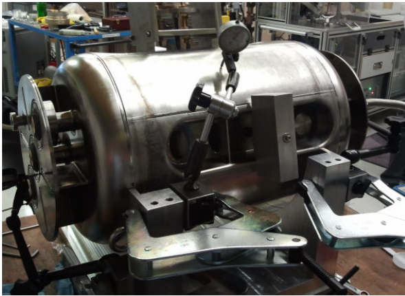
Figure 6: Setup for pressure sensitivity measurement.
