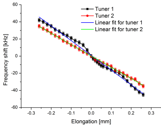
Figure 3: Frequency shift caused by elongation of tuner 1 and tuner 2.
