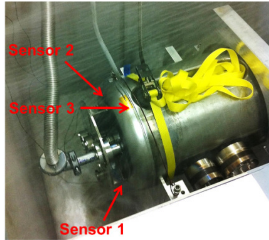
Figure 4: Setup for the preliminary cold test. Thermal sensors on top, alongside and bottom of the end cap.
