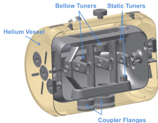
Figure 1: Layout of the superconducting 7-cell CH-Cavity (325.224 MHz, \beta = 0.16 ) [4].
