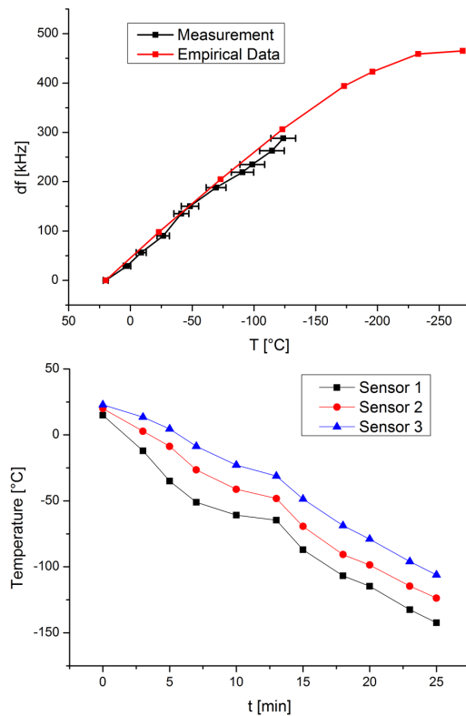
Figure 5: Top: Measured and expected frequency shift due to thermal shrinkage (Empirical data taken from: A.F. Clark, Materials at Low Temperatures). Bottom: Temperature behaviour for all three sensors.
