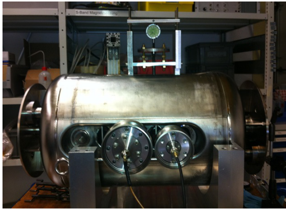
Figure 2: Setup for the test of the dynamic bellow tuners.
