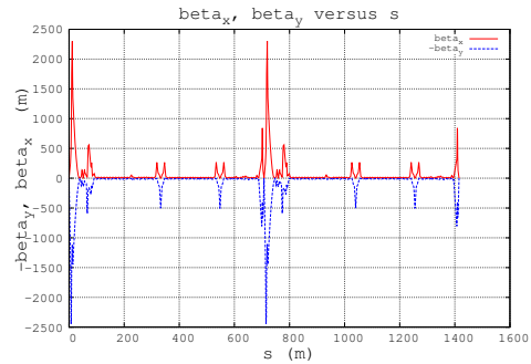
Figure 2: Betatron functions, horizontal and vertical.
