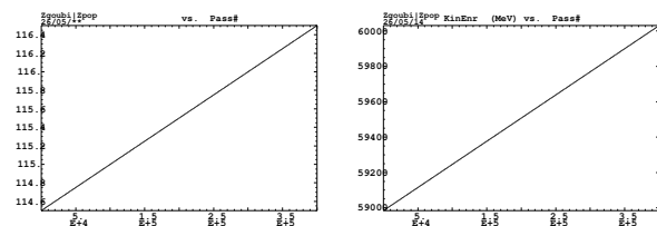
Figure 11: G\gamma (left) and kinetic energy (right) plotted vs. the turn number every 200 turns, over 400,000 turns. The particle is initially launched along the reference orbit in a ring with one of the arc dipoles rolled by 0.2 mrad.
