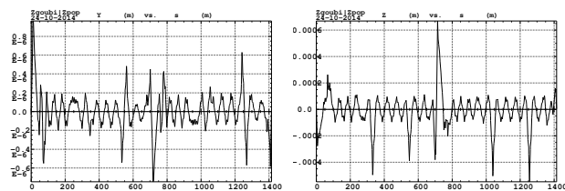
Figure 6: Closed orbits, horizontal and vertical, in the presence of a 0.2 mrad roll angle in an arc dipole.
