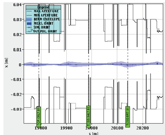
Figure 1: The IR7 horizontal aperture and beam orbit, with the envelope denoting the 1\text{-}\sigma beam size. The green text boxes show names of a few IR7 horizontal collimators.
