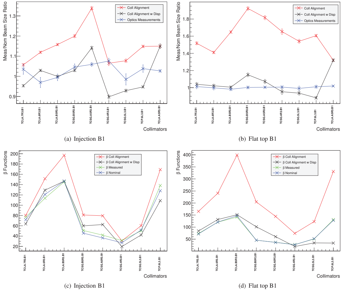
Figure 3: Beam size ratios and \beta -functions at injection and flat top for IR3 collimators.
