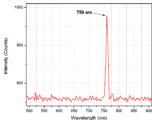
Figure 3: Lasing spectrum with the ERL operating with a positive momentum compaction. The losses for the 800 nm resonant wavelength were huge so the laser lased at a shorter wavelength where the losses were about 50% per pass.
