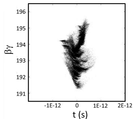
Figure 2: Compression in a system with negative momentum compaction (a) with strong CSR can lead to an incompressible longitudinal distribution, while compression in a system with positive momentum compaction (b) leads to a more compact phase space.
