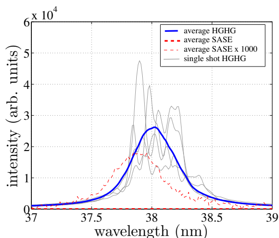
Figure 4: Average of 1000 FEL spectra for HGHG operation (blue solid line) and typical single-shot spectra at the mean pulse energy with HGHG seeding (thin line). The SASE background (red dashed lines) was multiplied by a factor of 1000 for better visibility.
