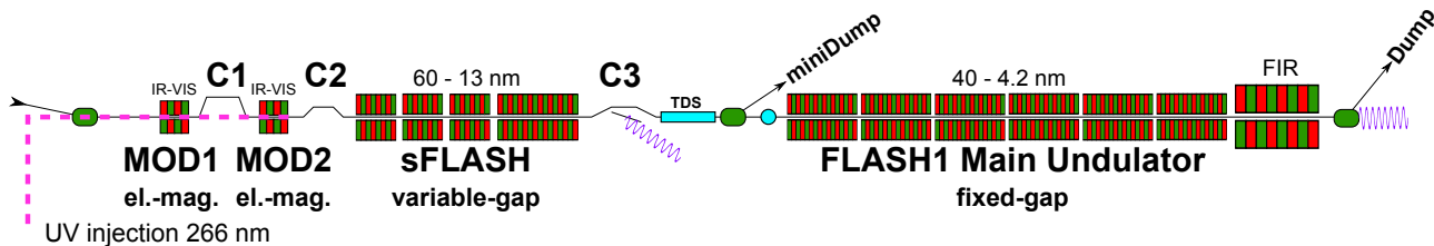
Figure 1: Layout of the FLASH1 beamline.
