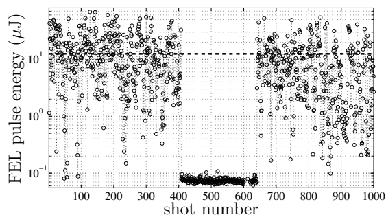
Figure 3: FEL pulse energy of 1000 consecutive shots. Between shot number 400 and 650, the seed laser shutter was closed.
