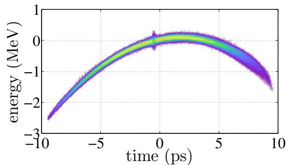
Figure 2: Longitudinal phase-space distribution measured after the seeding setup for an uncompressed electron bunch. The laser-induced energy modulation emerges as a region with larger slice energy spread.
