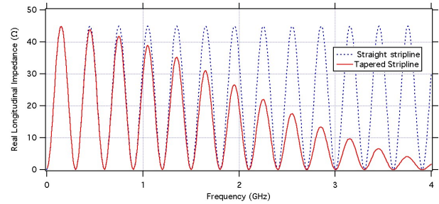
Figure 4: Real longitudinal impedance. Comparison of tapered and untapered striplines, same total length.
