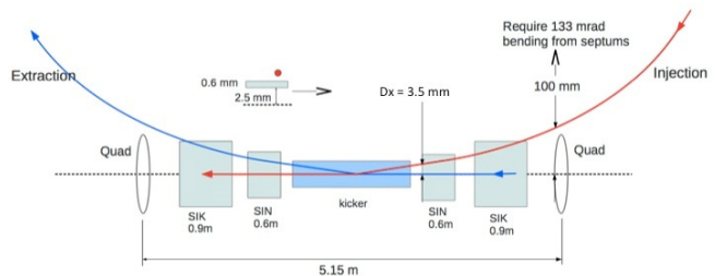
Figure 1: Layout of the ALS-U lattice in the injection/extraction straight.
