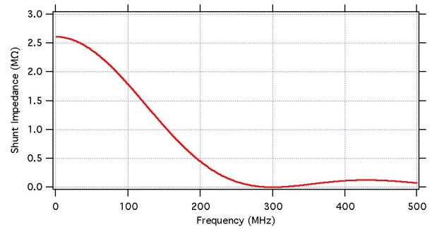
Figure 2: Stripline kicker module shunt impedance.
