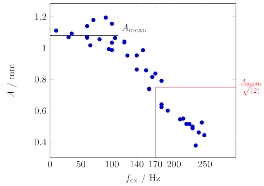
Figure 4: Bandwidth of the complete correction system: shown is the amplitude A of the orbit response when exciting a steering magnet with f_{\text{ext}} .
