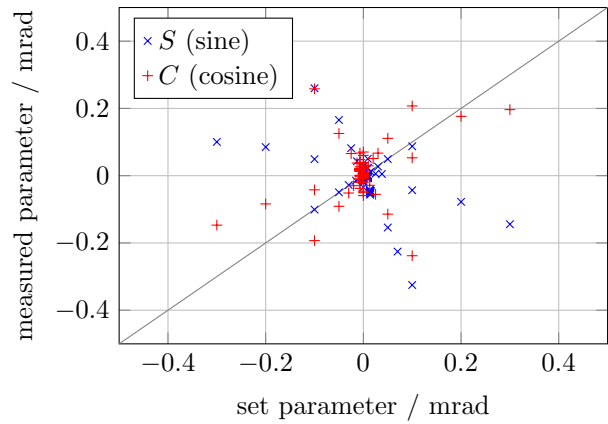
Figure 3: Parameters of the previous harmonic correction scheme for \gamma a = 3, 4, 5 . They deviate from the set parameters due to the quadrupole contributions caused by the orbit response to the correction fields.
