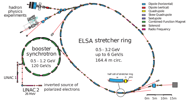
Figure 1: The Electron Stretcher Facility ELSA in Bonn.
