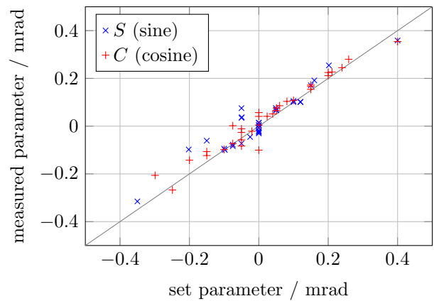
Figure 5: Parameters of the improved harmonic correction scheme for \gamma a = 3, 4, 5 . They are consistent with the set parameters, because the orbit response is included in the calculation of the correction fields.
