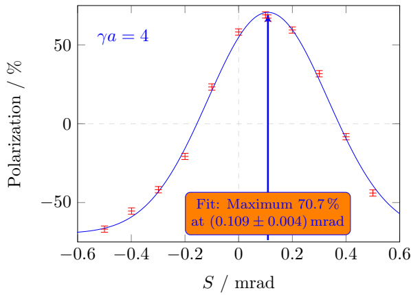
Figure 2: Møller polarimeter measurement from polarization optimization of integer resonance \gamma a = 4 in March 2014. It took about 10 min to obtain one polarization value with a statistical error of 2 %. A Gaussian fit is used to determine the maximum.
