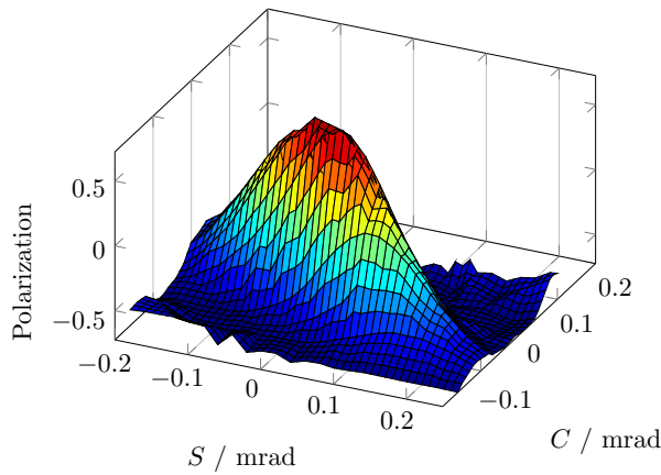
Figure 4: Simulation of the optimization of \gamma a = 6 with the previous harmonic correction scheme. The consecutive optimization of both correction parameters may not result in the global maximum of polarization.
