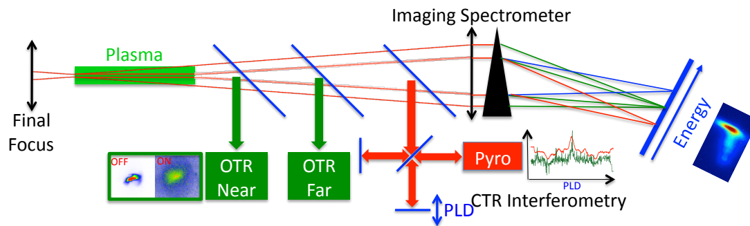
Figure 1: Schematic of the E209 experiment at SLAC FACET. The beam ( e^- or e^+ ) is focused near the entrance of the plasma. The plasma is created by laser photo-ionization of a metallic vapor (lithium) [9] (not shown). The time integrated bunch transverse profile can be recorded \sim 1 and \sim 2 m downstream from the plasma exit using optical transition radiation (OTR). Coherent transition radiation (CTR) interferometry is performed \sim 3 m downstream from the plasma exit using a Mach-Zender interferometer and a pyro-electric detector. The bunch energy spectrum can be recorded by an imaging magnetic spectrometer. Figure not to scale.
