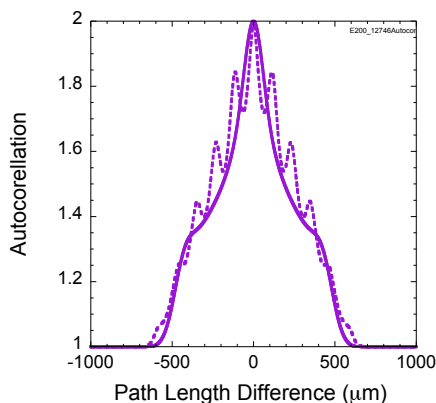
Figure 4: Calculated autocorellation traces for the un-modulated bunch profile of Fig. 2 (continuous line) and for the calculated model profile of Fig. 3 (dashed line).
