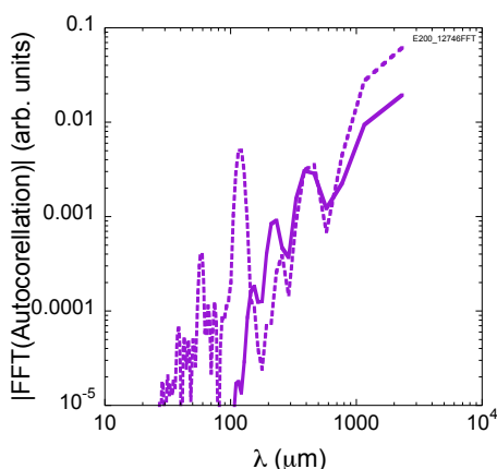
Figure 5: Fourier spectra of the autocorellation traces for the un-modulated bunch profile (continuous line) and for the calculated model profile (dashed line) of Fig. 4. Both traces are normalized to 2.
