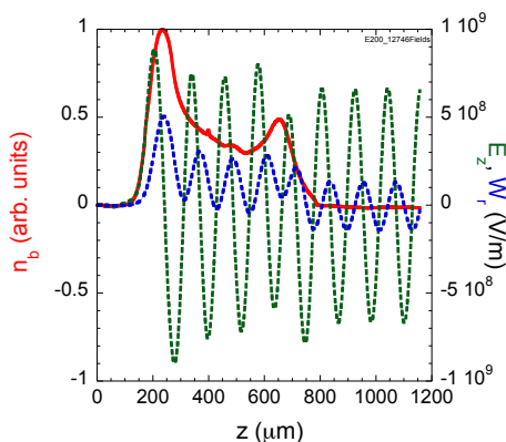
Figure 2: An example of the bunch longitudinal density profile measured recently (red line). The bunch propagates towards the left. The corresponding longitudinal: E_z , green dashed line, and transverse: W_r , blue dashed line, wakefields.
