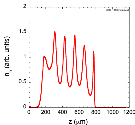
Figure 3: Bunch density profile obtained by assuming that the transverse wakefields lead to the longitudinal profile given by: n_b = n_{b0}/(W_r/\max(W_r) + 0.3) . The bunch propagates towards the left.
