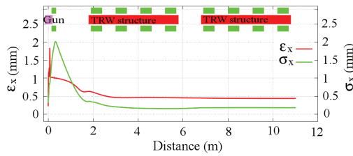
Figure 4: Horizontal emittance and beam size through the injector.
