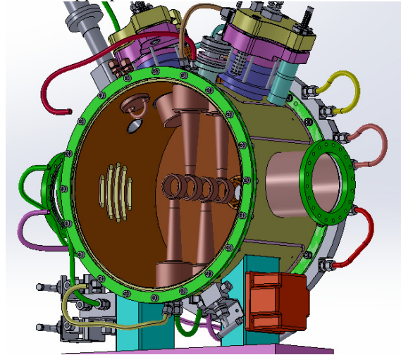
Figure 1: 3D model of the re-buncher cavity.
