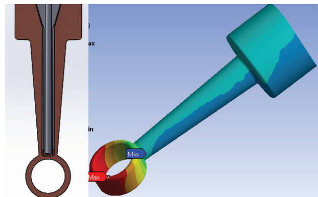
Figure 5: stems cooling overview (left) and calculated temperature distribution on a side stem (right).
