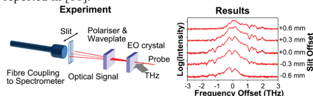
Figure 8: Alignment dependent distortions in EO up-conversion signal measured through aperture offsets [11].
