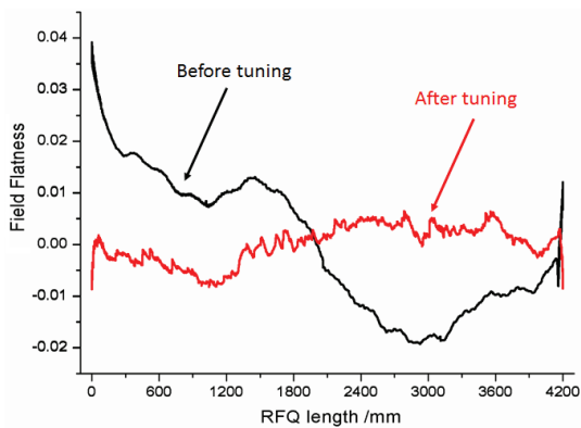
Figure 3: Field flatness before and after tuning.
