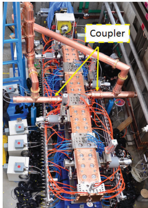
Figure 4: The injector II RFQ on site.
