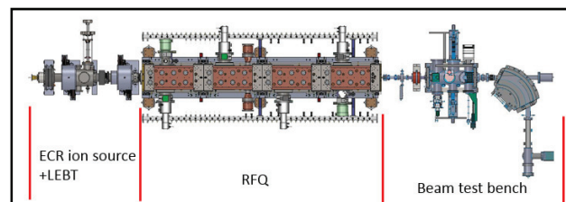
Figure 6: The injector II RFQ acceleration system.
