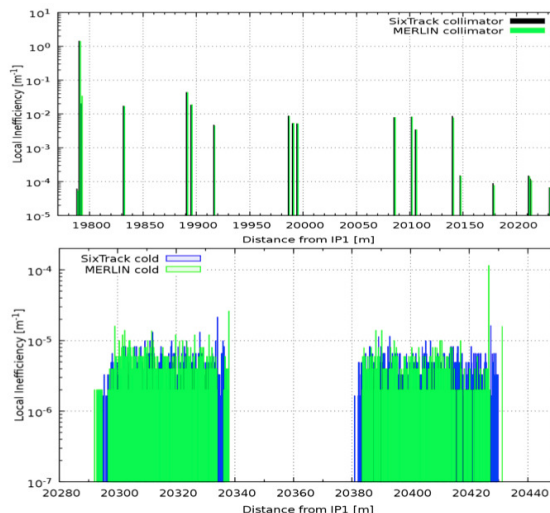
Figure 4: Collimator loss comparison in IR7(top): SixTrack in black and MERLIN in green. Cold Losses comparison in the dispersion suppressor downstream IR7(bottom): SixTrack in blue and MERLIN in green.
