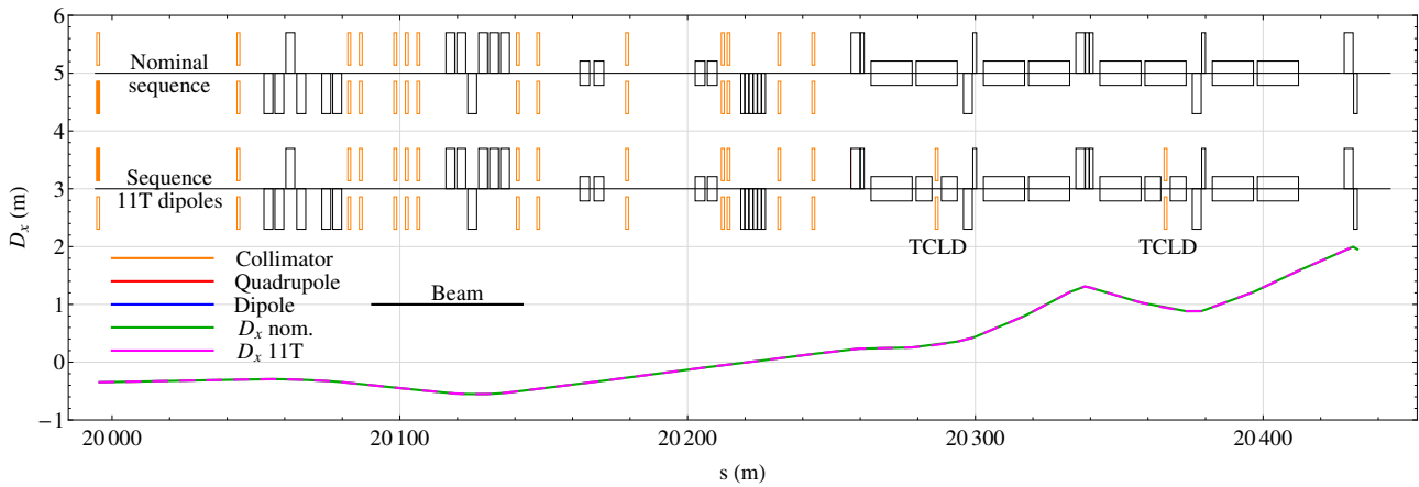
Figure 1: Layout of a part of IR7 with the nominal sequence (top) and with two main dipoles replaced by 11 T dipole assemblies with a TCLD collimator in between (middle). The dispersion function for the two cases, using nominal optics, is also shown.
