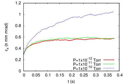
Figure 7: Evolution of the horizontal emittance during the bunching process prior to extraction with cooling for different levels of vacuum pressure in the beam pipe.
