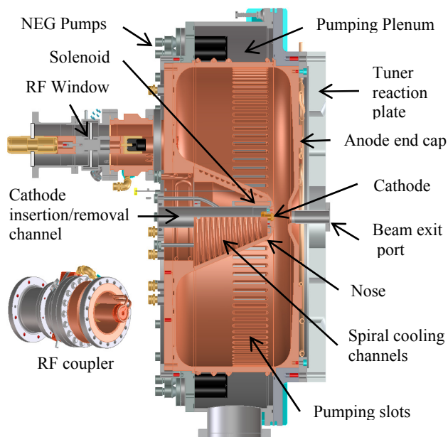
Figure 1: VHF Gun in cross section.
