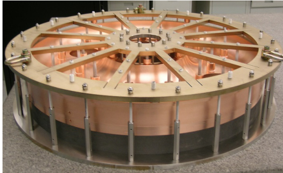
Figure 3: Cathode end cap in brazing fixture.
