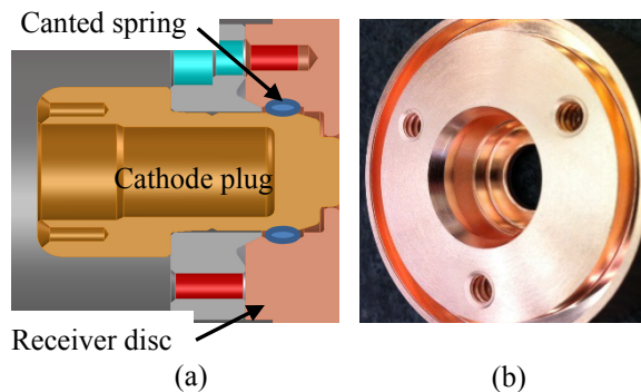
Figure 2a: CAD Model of cathode plug region, 2b: photo of cathode receiver.
