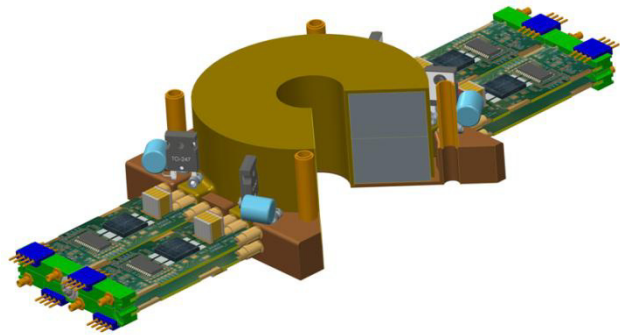
Figure 6. CAD model of single stage of the conventional inductive adder showing the cross-section of the ferrite core.
