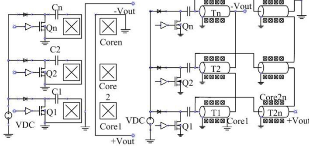
Figure 4. Simplified schematics of an inductive adder on the left, and a transmission line adder on the right.
