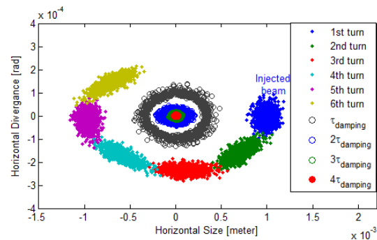
Figure 2: Evolution of the injected beam with an offset in phase space of ALS-U lattice at injection point.
