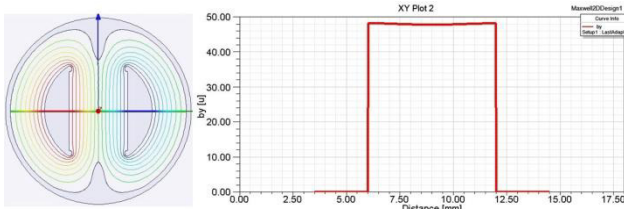
Figure 3. Cross section and flux of the magnet on the left and B field on the right.
