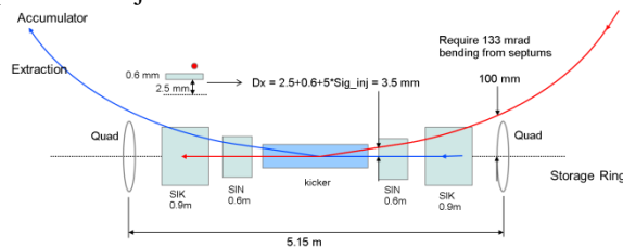
Figure 1 Schematic of swap-out injection.
