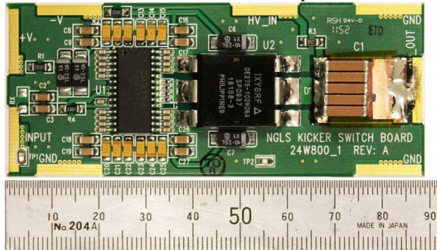
Figure 5. Photo of MOSFET switch circuit.
