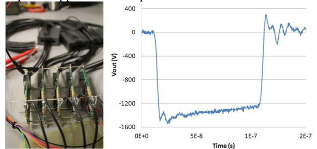
Figure 7. Five cell transmission line adder and output pulse into 50 \Omega .
