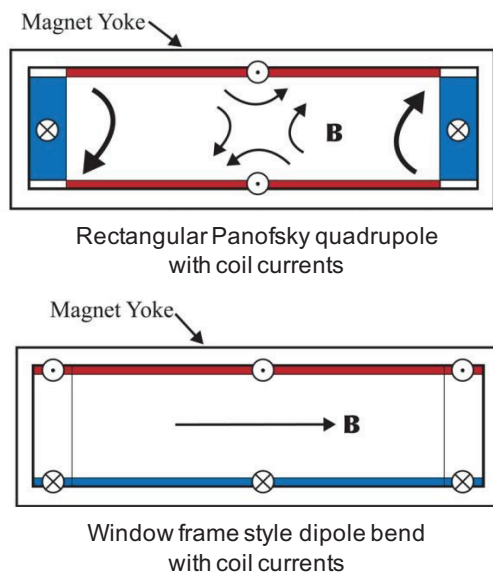
Figure 4: Quadrupole and Dipole Current Flows [7].
