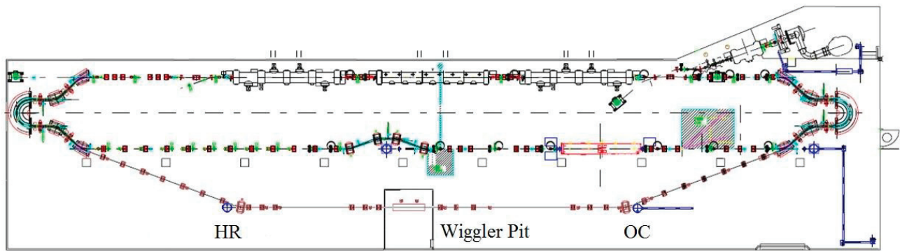
Figure 1: JLab IR and UV FELs in facility, showing SRF linac (top), IR recirculator (middle) and UV recirculator (bottom). The UV High Reflector vacuum vessel (HR), wiggler pit, and UV Out-Coupler (OC) locations are indicated.
