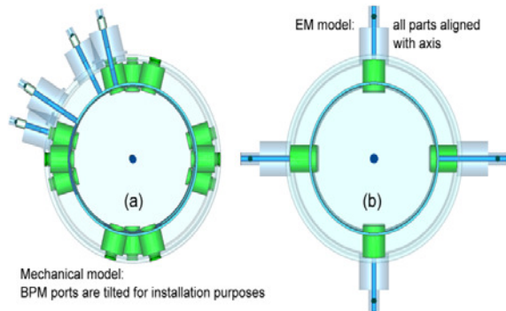
Figure 2: Transverse cross-sections, highlighting the difference in the mechanical and EM design.
