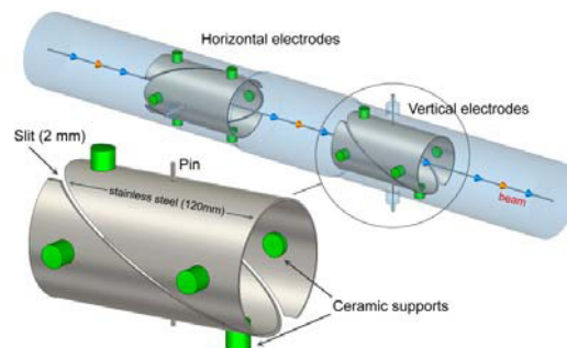
Figure 1: A simplified 3D model of the ELENA BPM.
