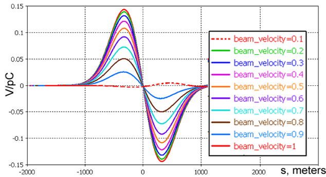
Figure 5: Longitudinal wake potential of the ELENA BPM as a function of \beta .
