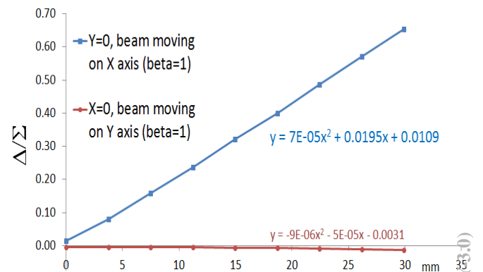
Figure 3: Signal linearity of horizontal electrodes to beam displacement in X and Y axis.
