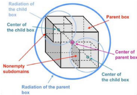
Figure 7: Boxes in the near and far zones according to the one-box-buffer scheme [4].
