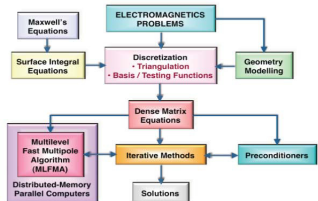
Figure 6: A typical simulation environment based on MLFMA [3].
