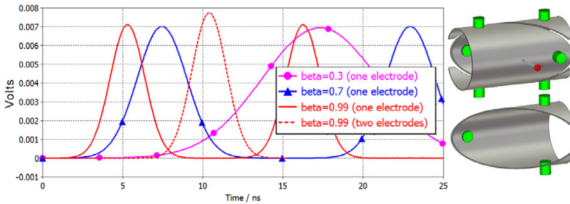
Figure 4: Simulated BPM signal in Volts as function of time for different betas; simplified pickup geometry.
